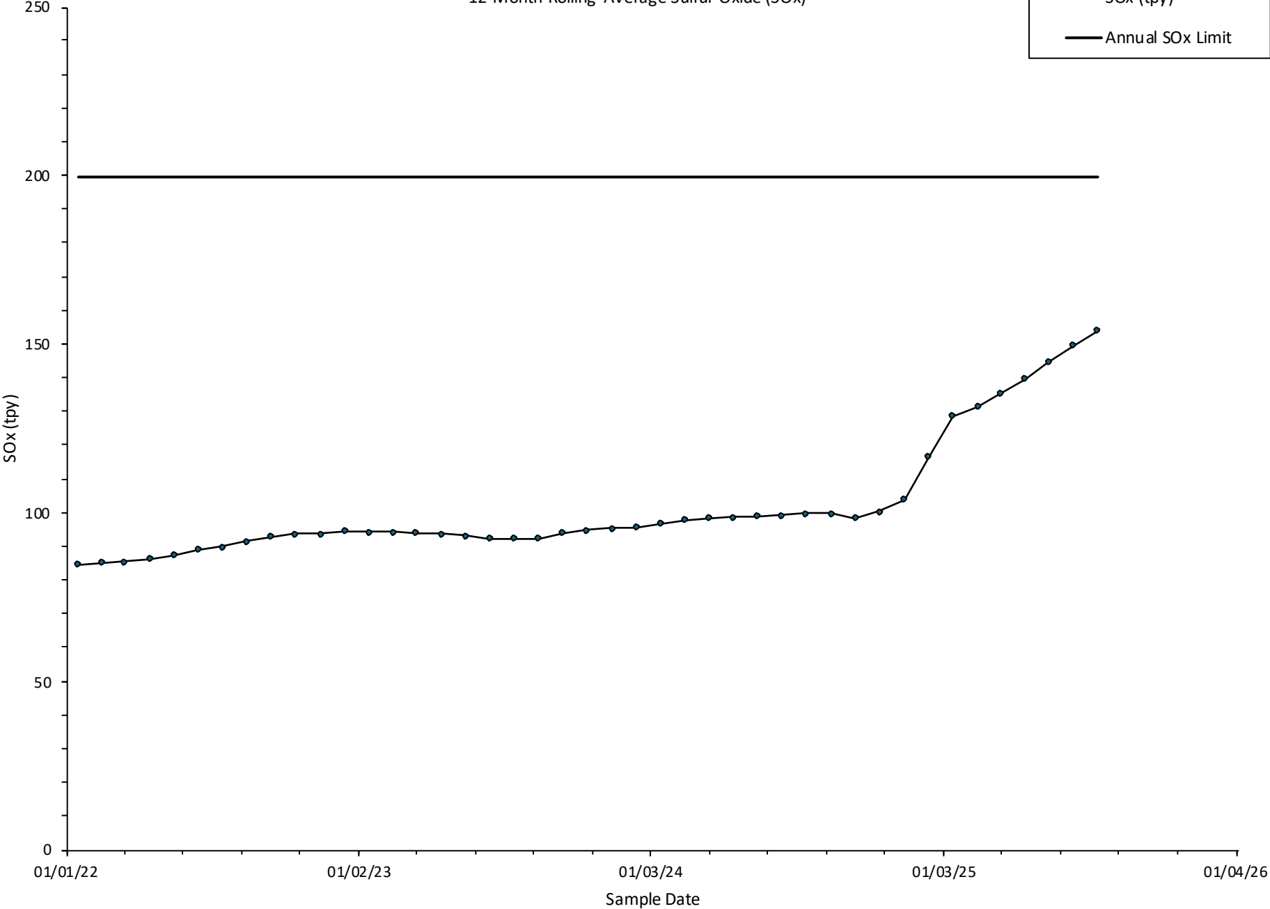
Air Emissions from Landfill Gas Combustion 12-Month Rolling Average Sulfur Oxide (SOx)
